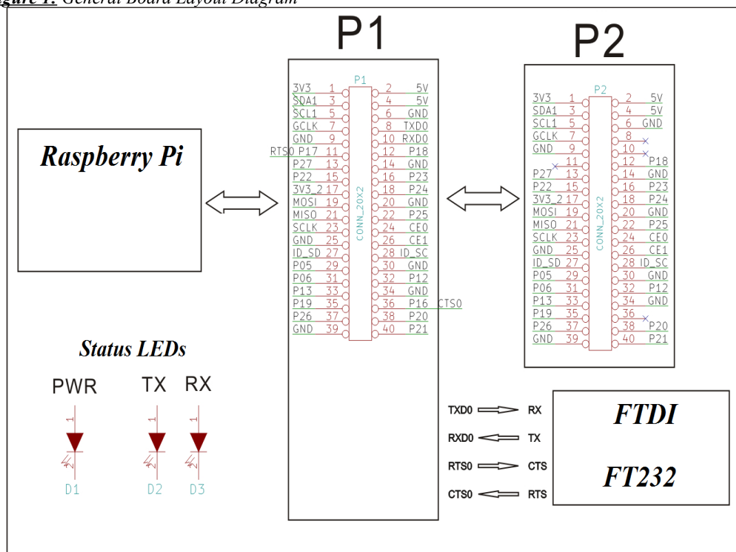
Figure 1: General Board Layout Diagram
